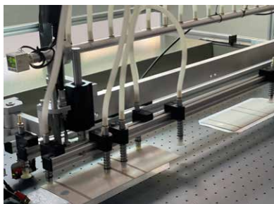
Case-Making Machine
